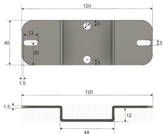
Figure 3. Sensor mounting adapter for TAC-B 4G
