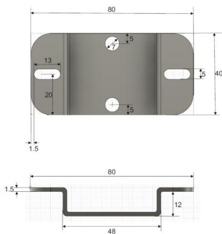
Figure 2. Sensor mounting adapter for TAC-B WP
